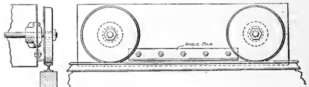
ANGLE BAR PREVENTS FALLING OF CRANE
